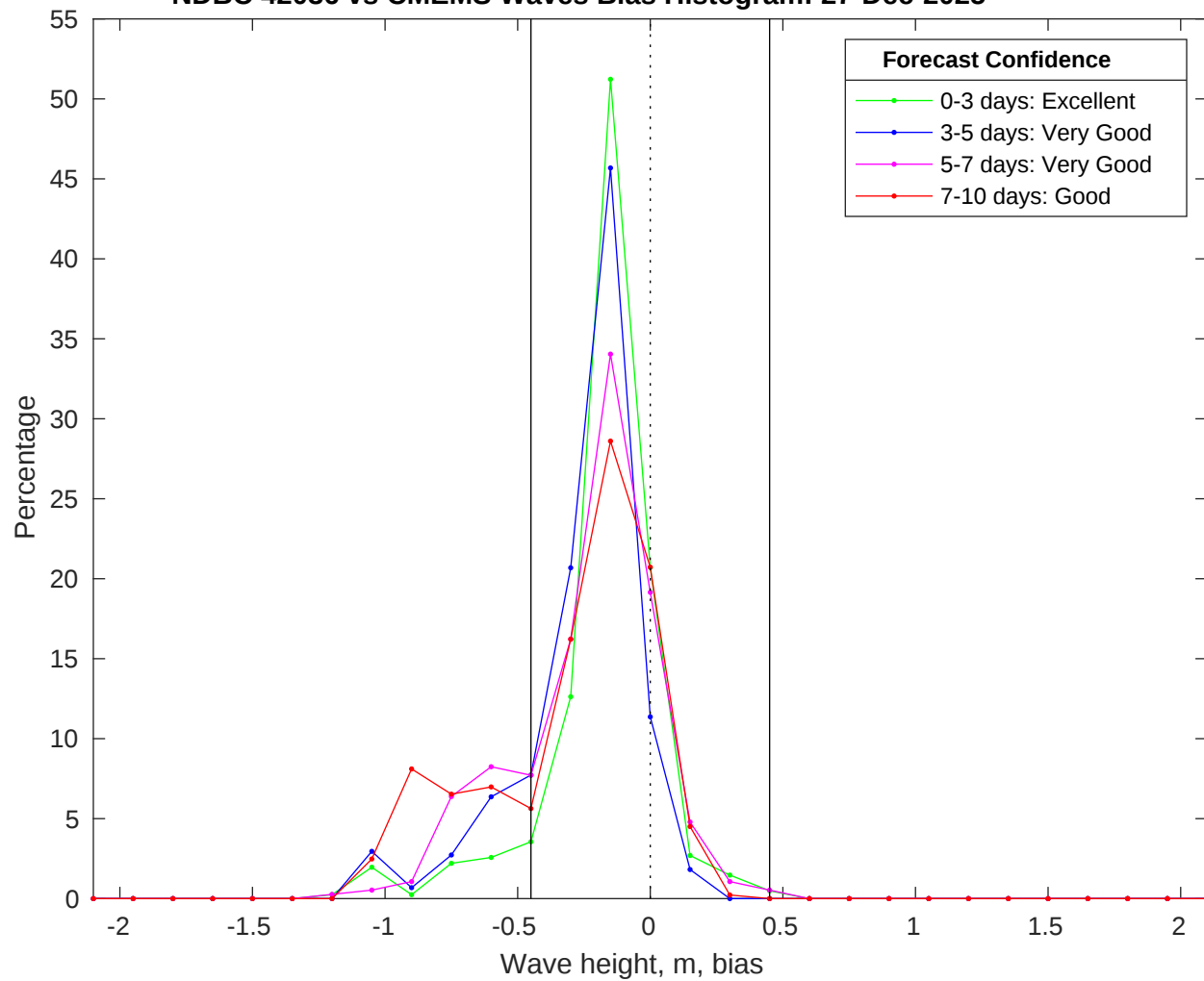
NDBC 42036 vs CMEMS Waves Bias Histogram: 27-Dec-2025
