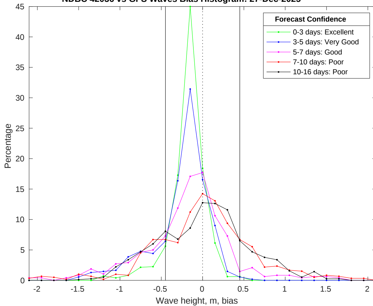
NDBC 42036 vs GFS Waves Bias Histogram: 27-Dec-2025
