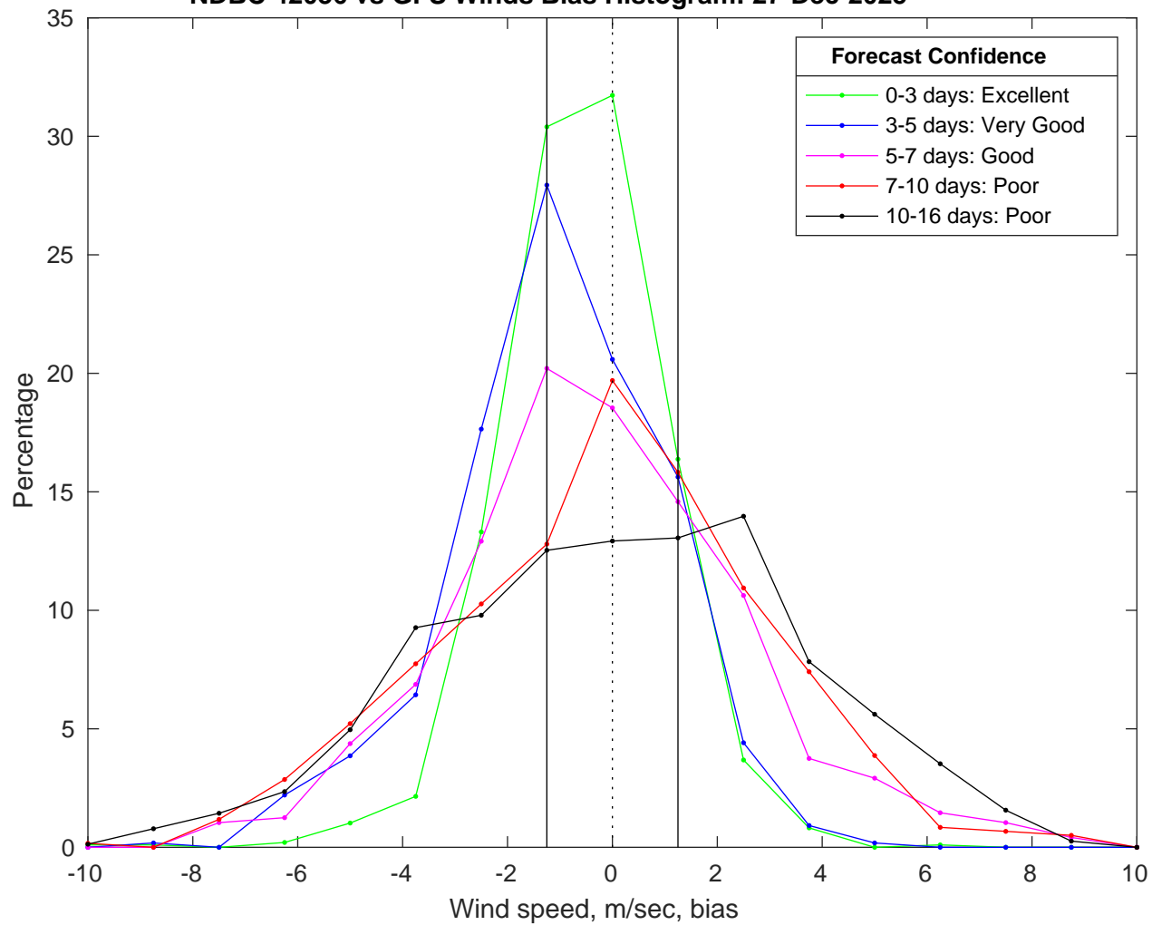
NDBC 42036 vs GFS Winds Bias Histogram: 27-Dec-2025
