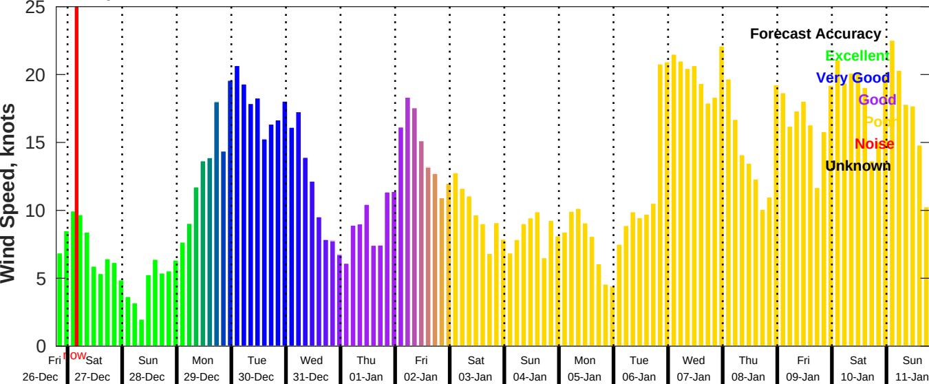
GFS Wind Speed Forecast for NDBC 42036 from 26-Dec-2025 19:00:00 to 11-Jan-2026 19:00:00
