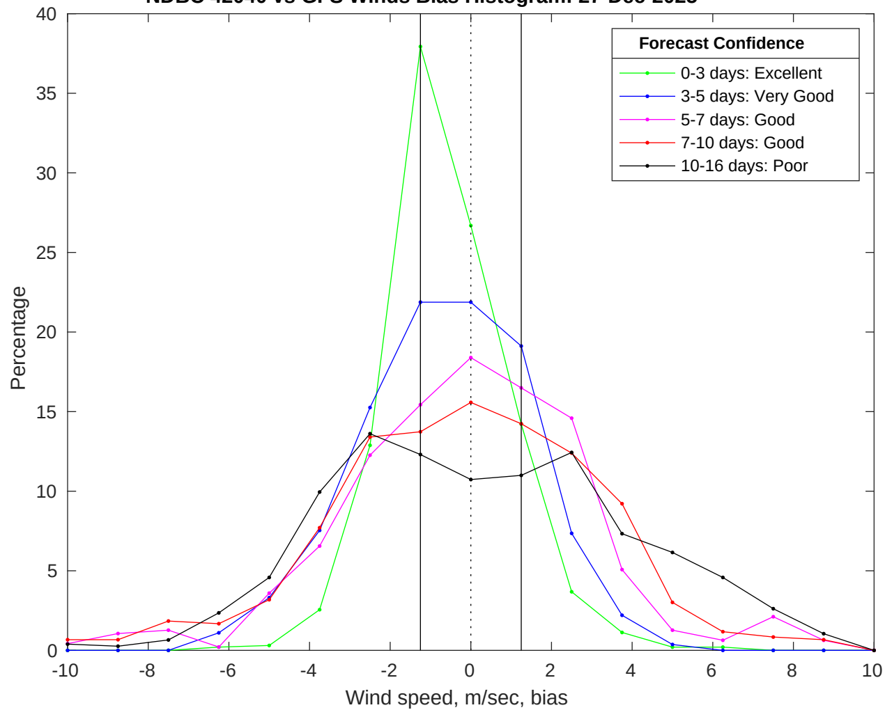
NDBC 42040 vs GFS Winds Bias Histogram: 27-Dec-2025
