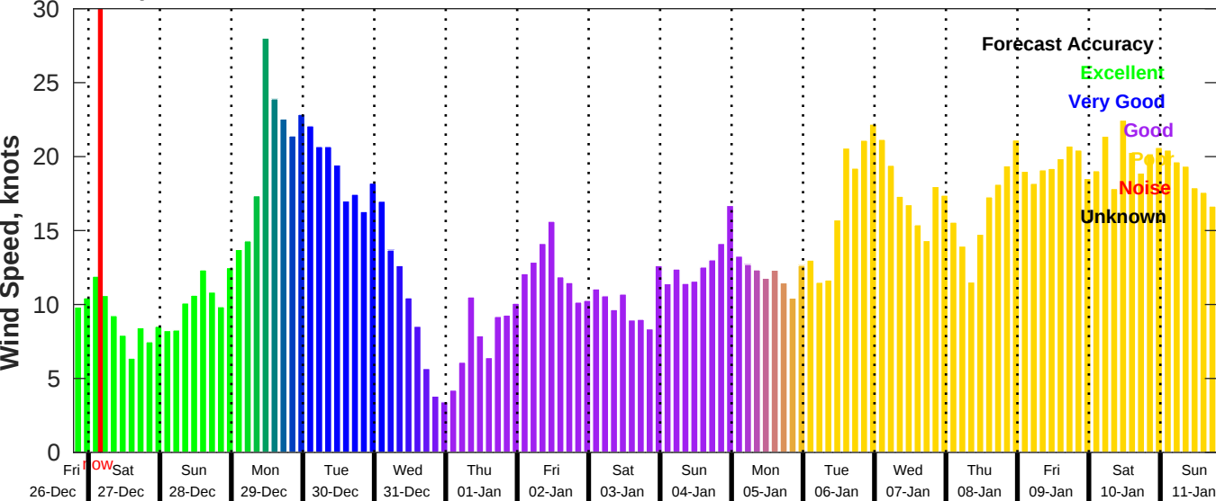
GFS Wind Speed Forecast for NDBC 42040 from 26-Dec-2025 19:00:00 to 11-Jan-2026 19:00:00
