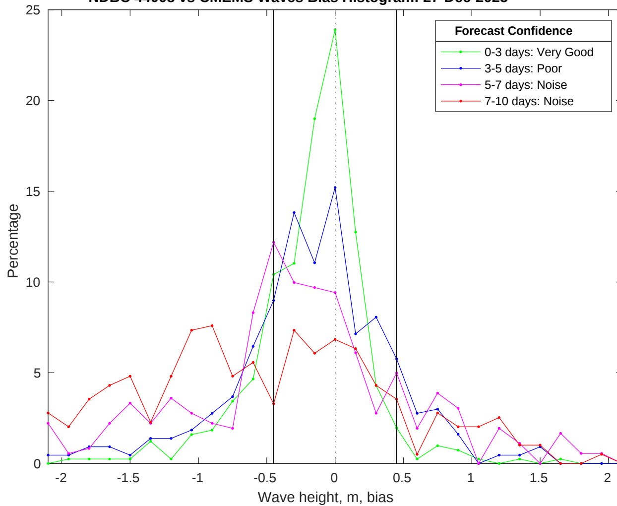
NDBC 44008 vs CMEMS Waves Bias Histogram: 27-Dec-2025
