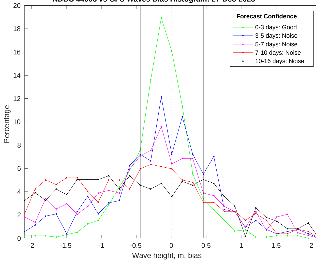
NDBC 44008 vs GFS Waves Bias Histogram: 27-Dec-2025
