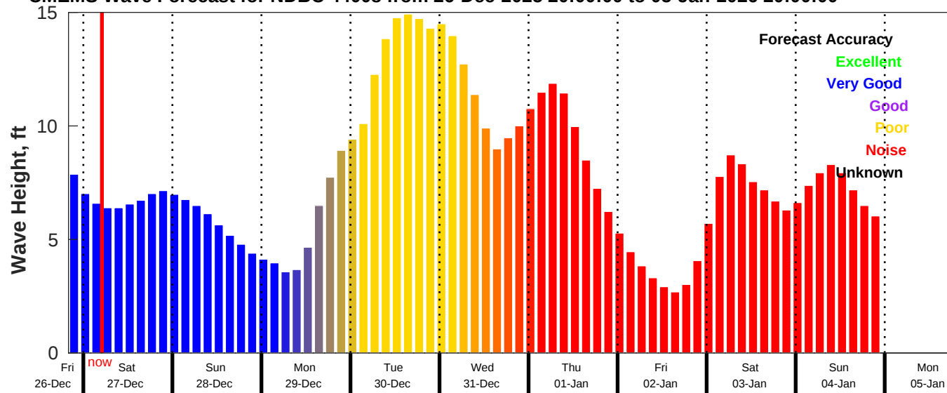
CMEMS Wave Forecast for NDBC 44008 from 26-Dec-2025 20:00:00 to 05-Jan-2026 20:00:00
