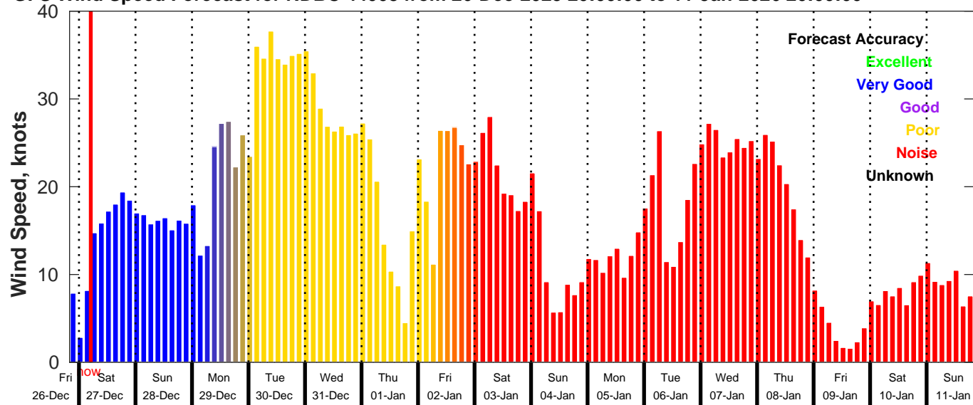
GFS Wind Speed Forecast for NDBC 44008 from 26-Dec-2025 20:00:00 to 11-Jan-2026 20:00:00
