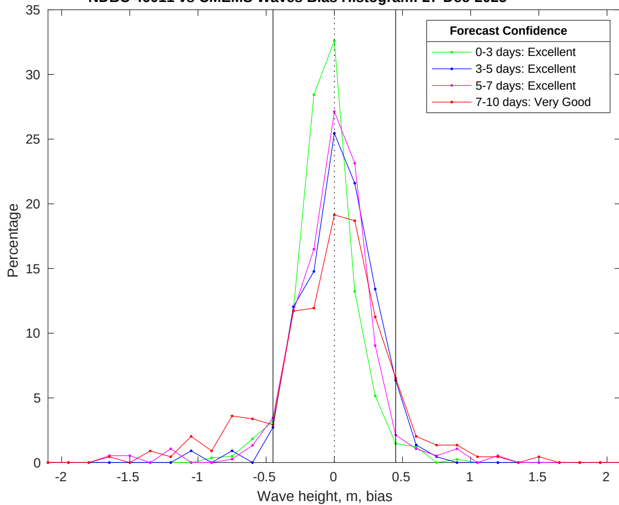
NDBC 46011 vs CMEMS Waves Bias Histogram: 27-Dec-2025
