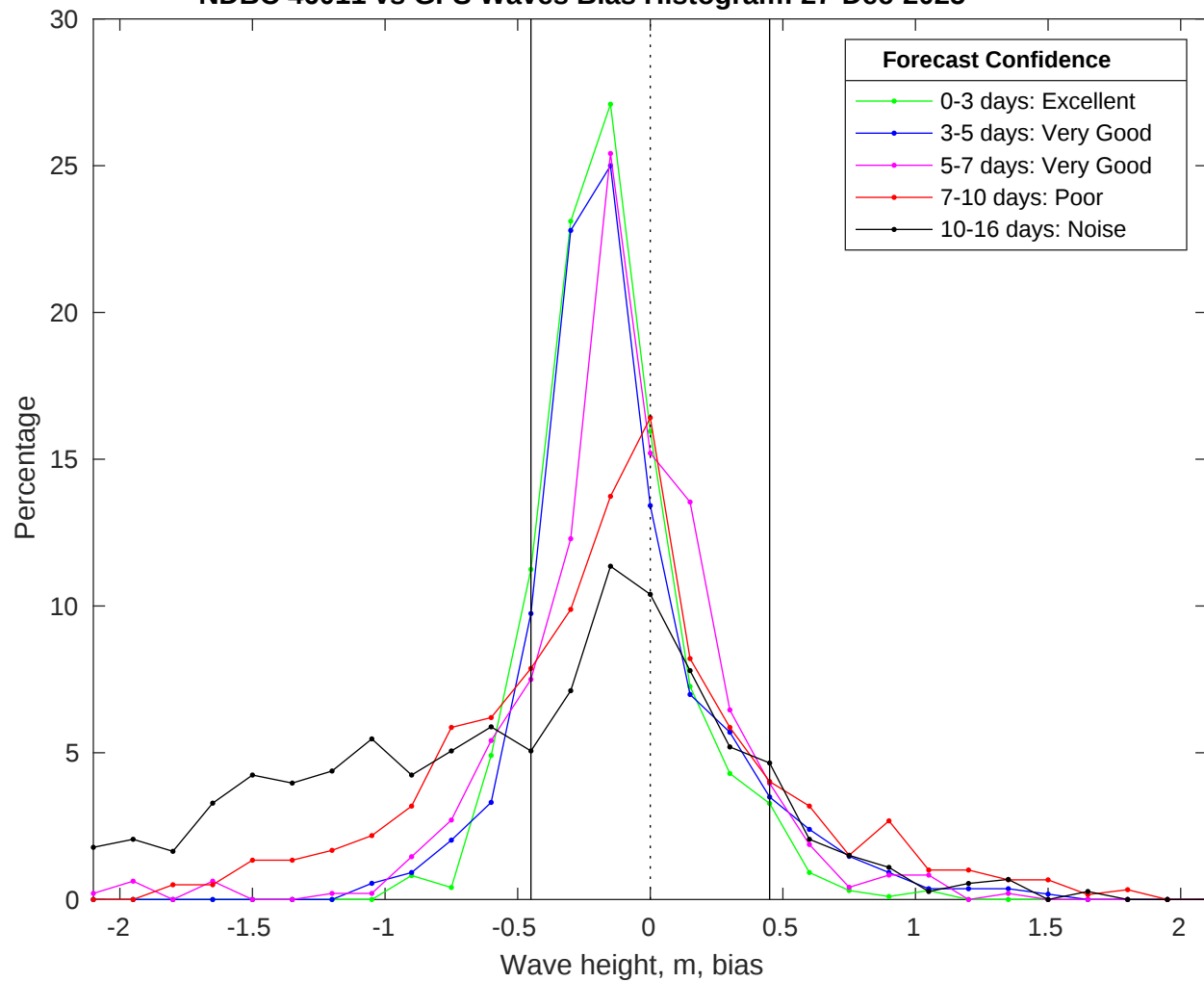
NDBC 46011 vs GFS Waves Bias Histogram: 27-Dec-2025
