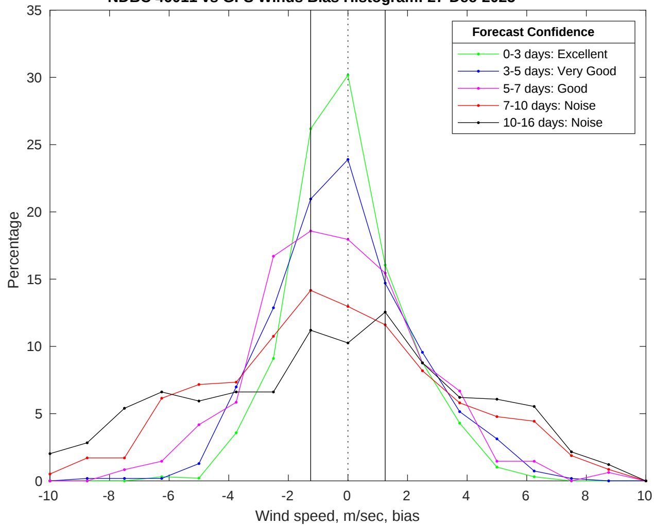
NDBC 46011 vs GFS Winds Bias Histogram: 27-Dec-2025
