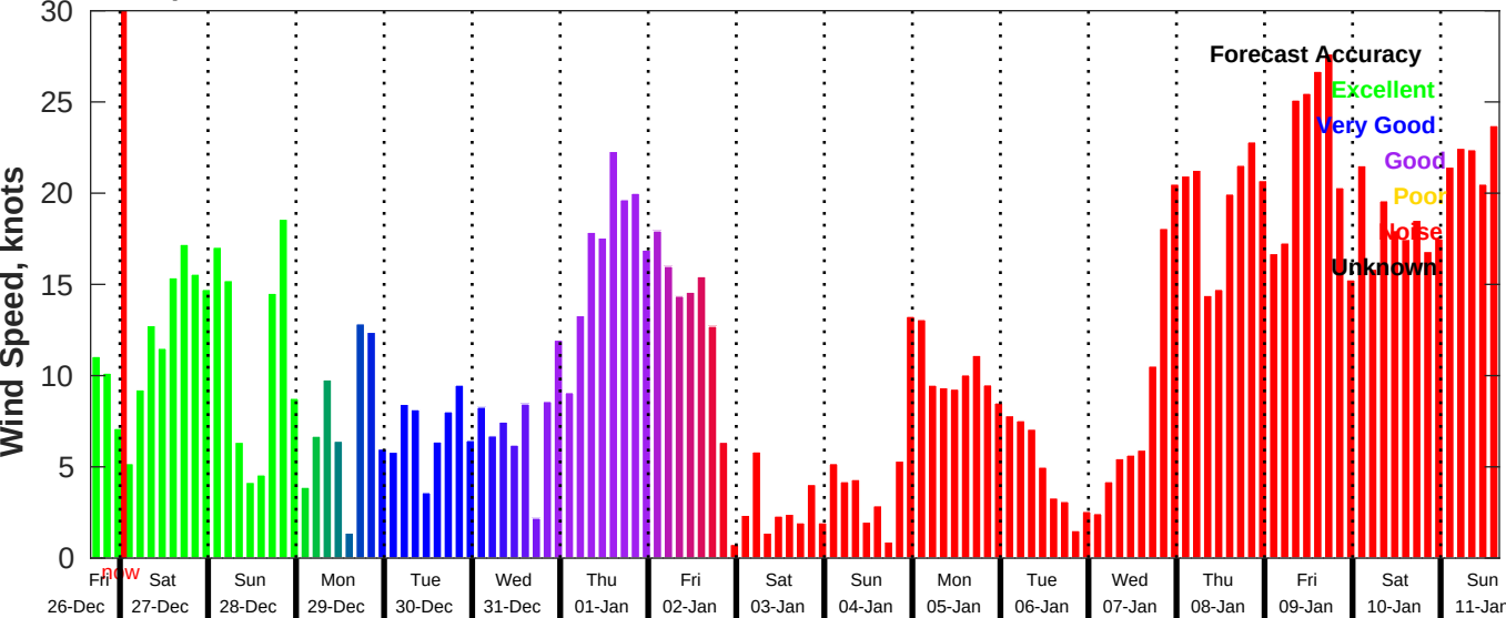
GFS Wind Speed Forecast for NDBC 46011 from 26-Dec-2025 16:00:00 to 11-Jan-2026 16:00:00
