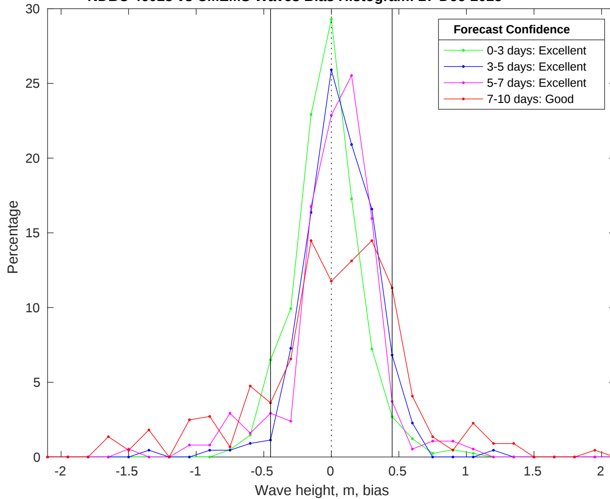
NDBC 46028 vs CMEMS Waves Bias Histogram: 27-Dec-2025
