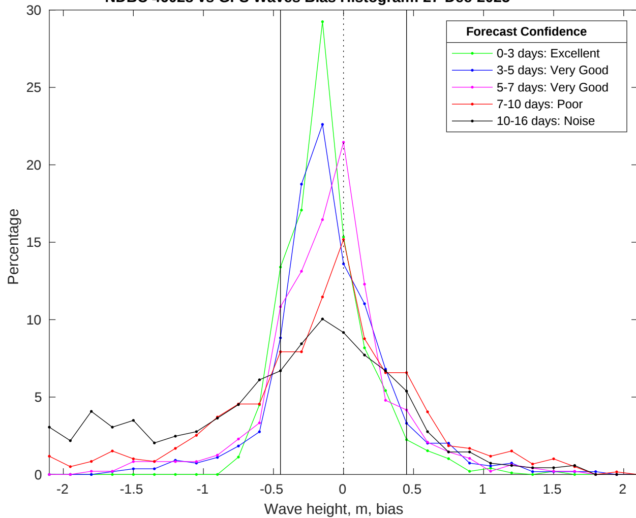
NDBC 46028 vs GFS Waves Bias Histogram: 27-Dec-2025
