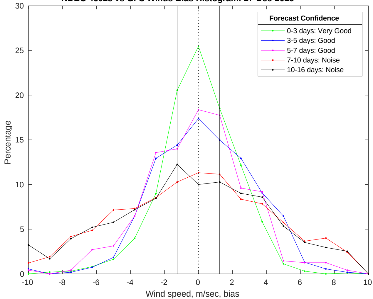
NDBC 46028 vs GFS Winds Bias Histogram: 27-Dec-2025
