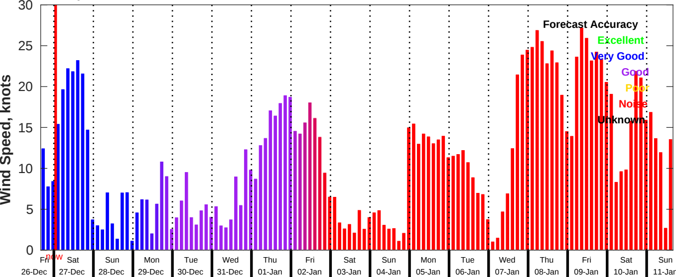
GFS Wind Speed Forecast for NDBC 46028 from 26-Dec-2025 16:00:00 to 11-Jan-2026 16:00:00
