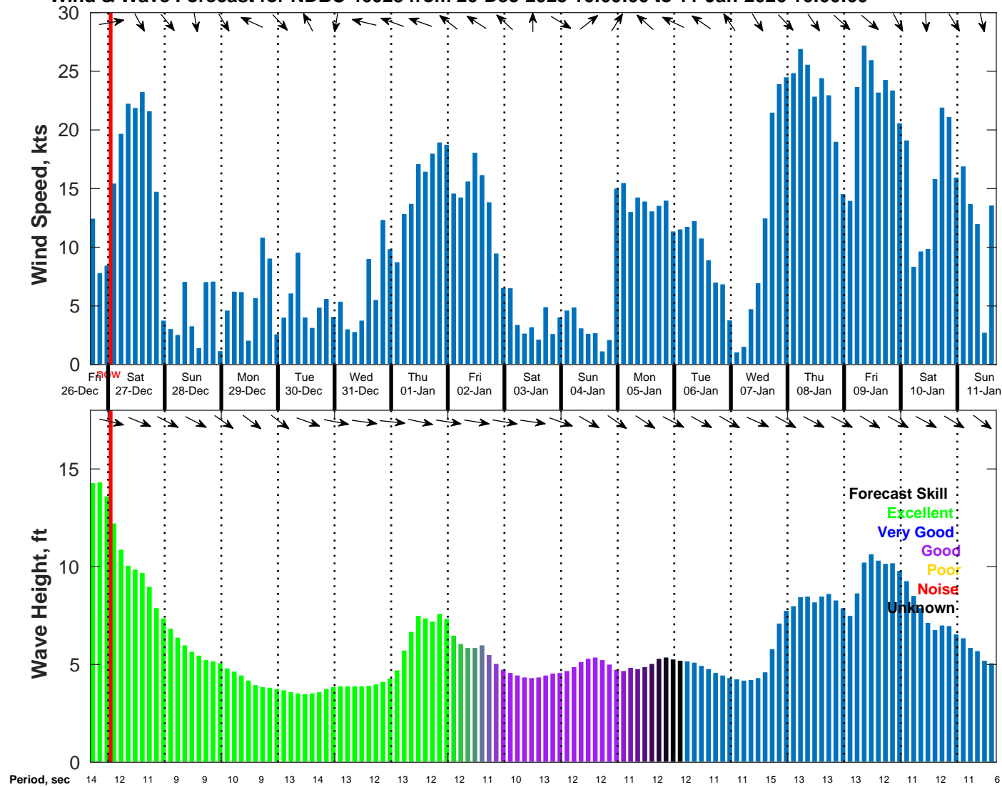
Wind & Wave Forecast for NDBC 46028 from 26-Dec-2025 16:00:00 to 11-Jan-2026 16:00:00
