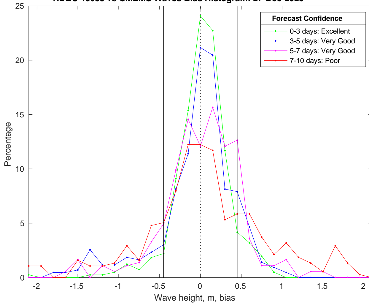
NDBC 46059 vs CMEMS Waves Bias Histogram: 27-Dec-2025
