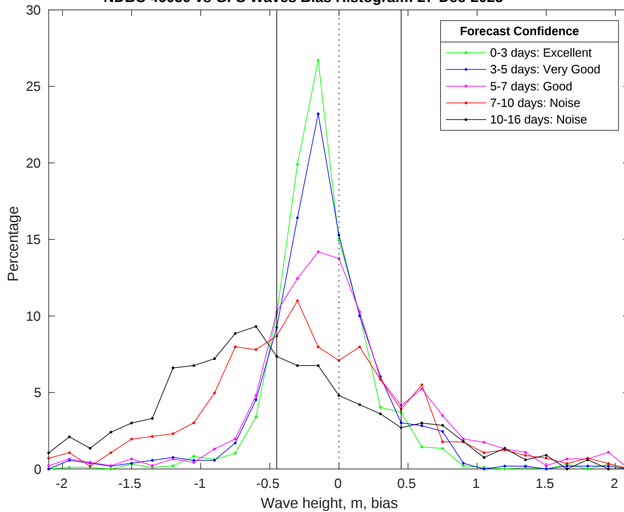
NDBC 46059 vs GFS Waves Bias Histogram: 27-Dec-2025
