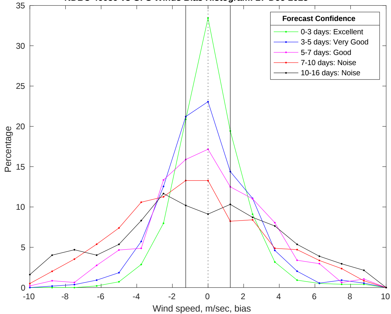
NDBC 46059 vs GFS Winds Bias Histogram: 27-Dec-2025
