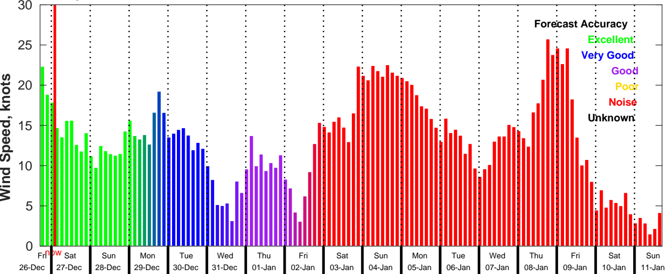
GFS Wind Speed Forecast for NDBC 46059 from 26-Dec-2025 17:00:00 to 11-Jan-2026 17:00:00
