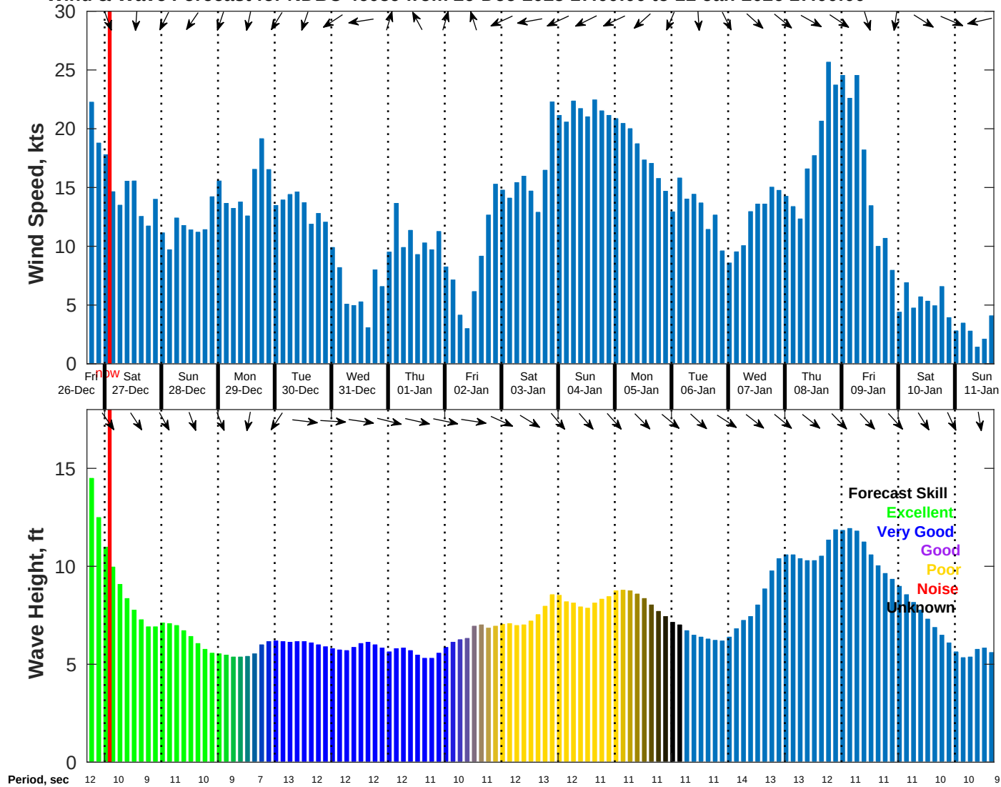
Wind & Wave Forecast for NDBC 46059 from 26-Dec-2025 17:00:00 to 11-Jan-2026 17:00:00
