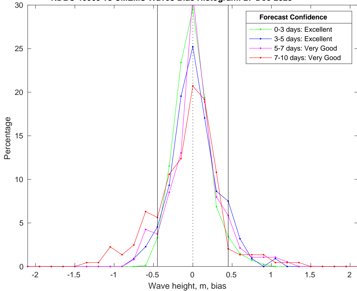
NDBC 46069 vs CMEMS Waves Bias Histogram: 27-Dec-2025
