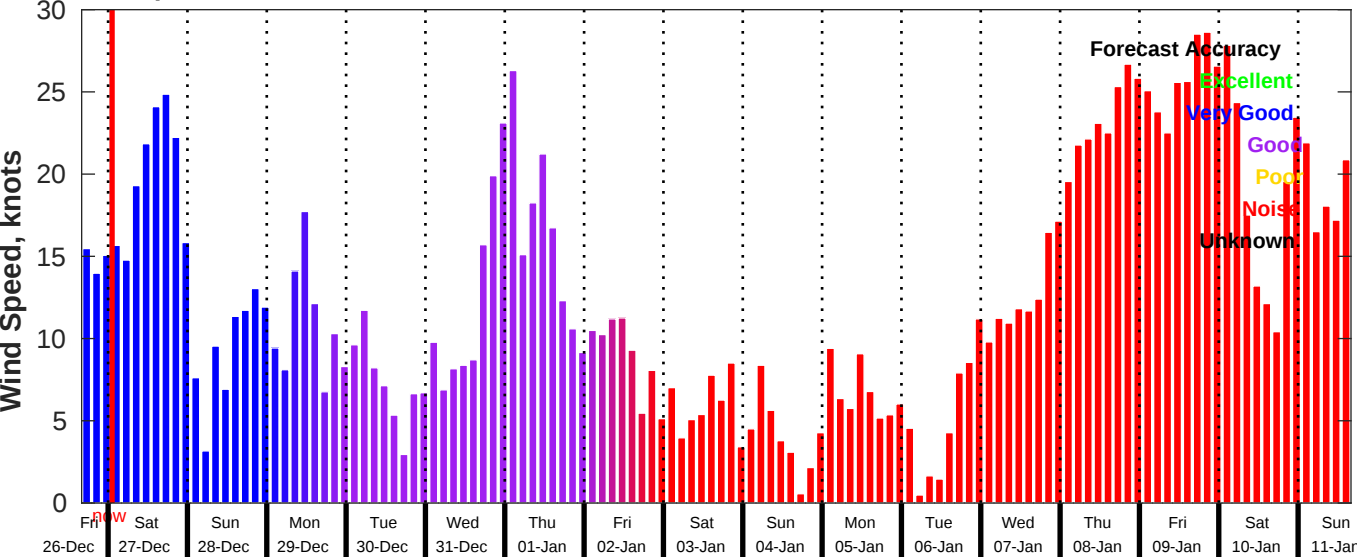
GFS Wind Speed Forecast for NDBC 46069 from 26-Dec-2025 16:00:00 to 11-Jan-2026 16:00:00
