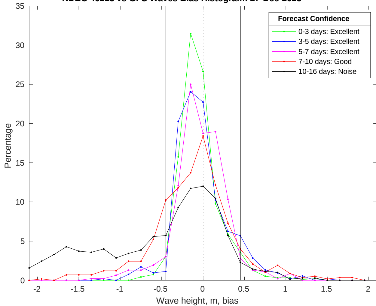
NDBC 46215 vs GFS Waves Bias Histogram: 27-Dec-2025
