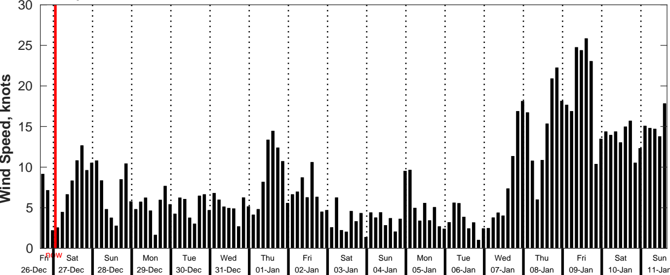
GFS Wind Speed Forecast for NDBC 46215 from 26-Dec-2025 16:00:00 to 11-Jan-2026 16:00:00
