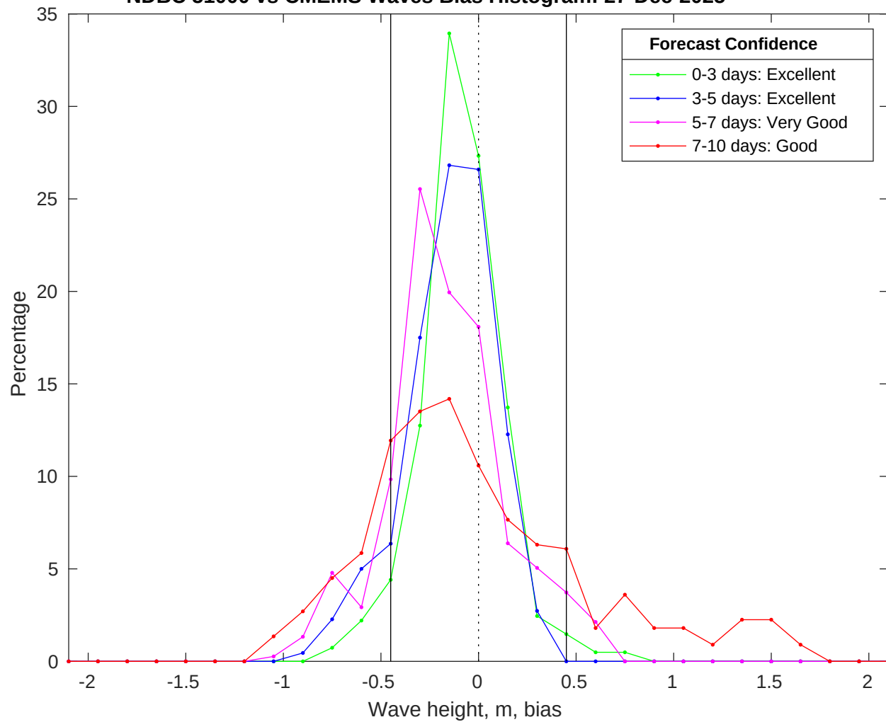
NDBC 51000 vs CMEMS Waves Bias Histogram: 27-Dec-2025
