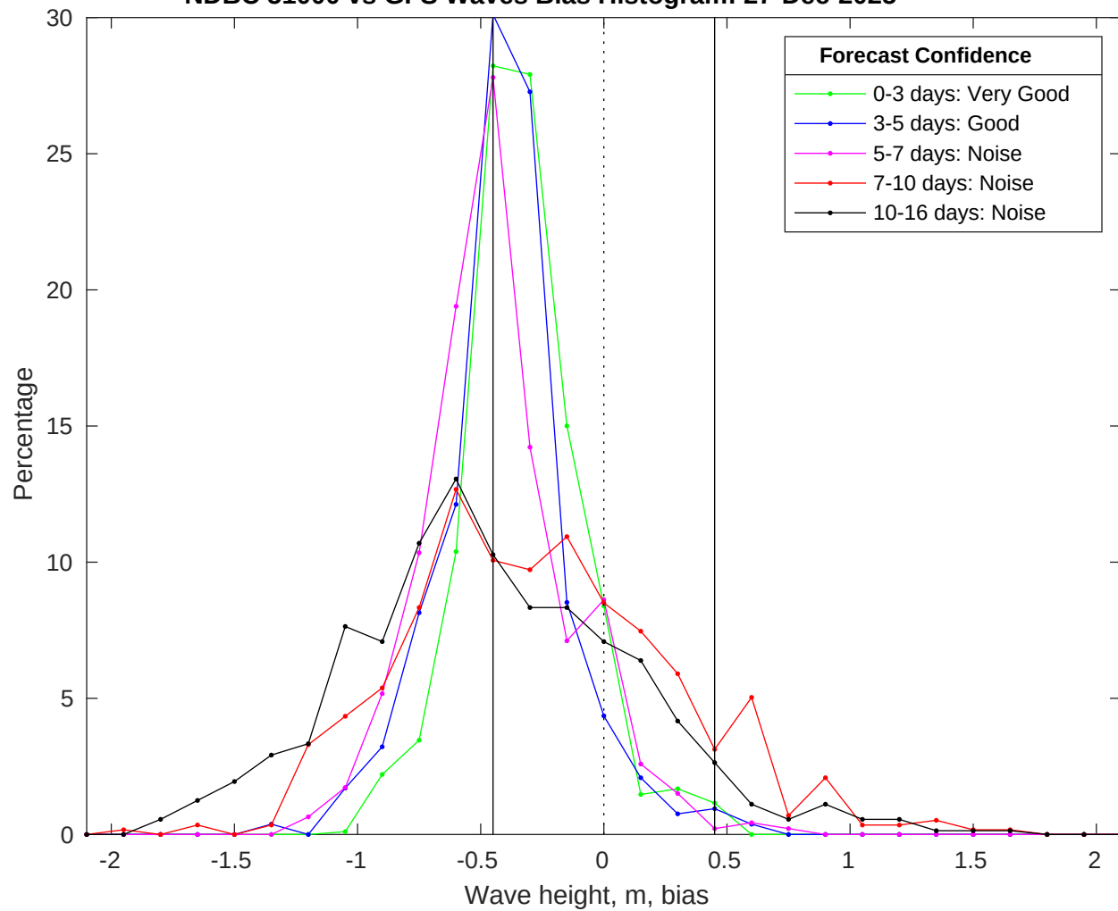
NDBC 51000 vs GFS Waves Bias Histogram: 27-Dec-2025
