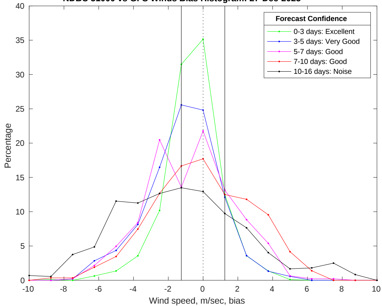
NDBC 51000 vs GFS Winds Bias Histogram: 27-Dec-2025
