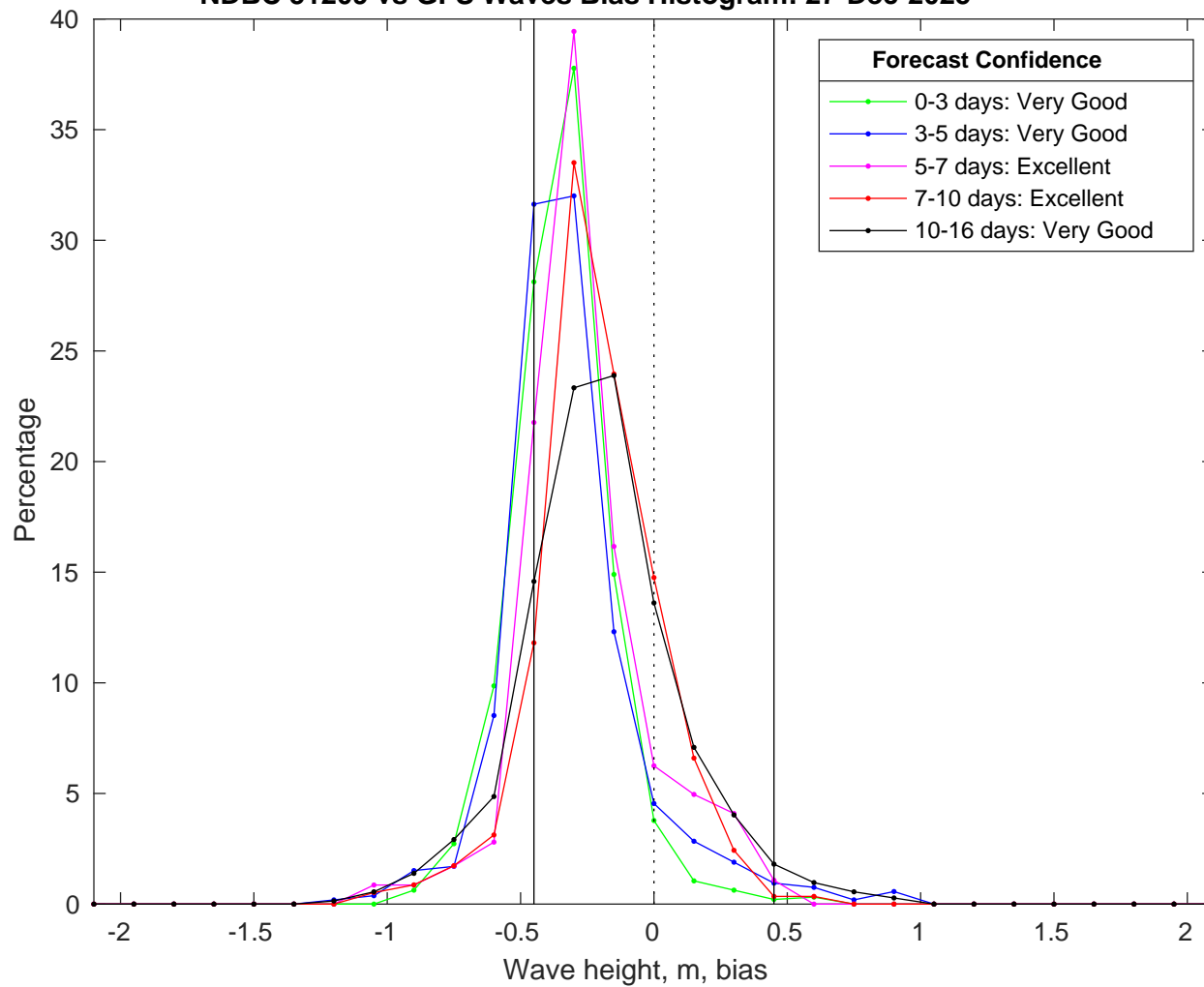
NDBC 51209 vs GFS Waves Bias Histogram: 27-Dec-2025
