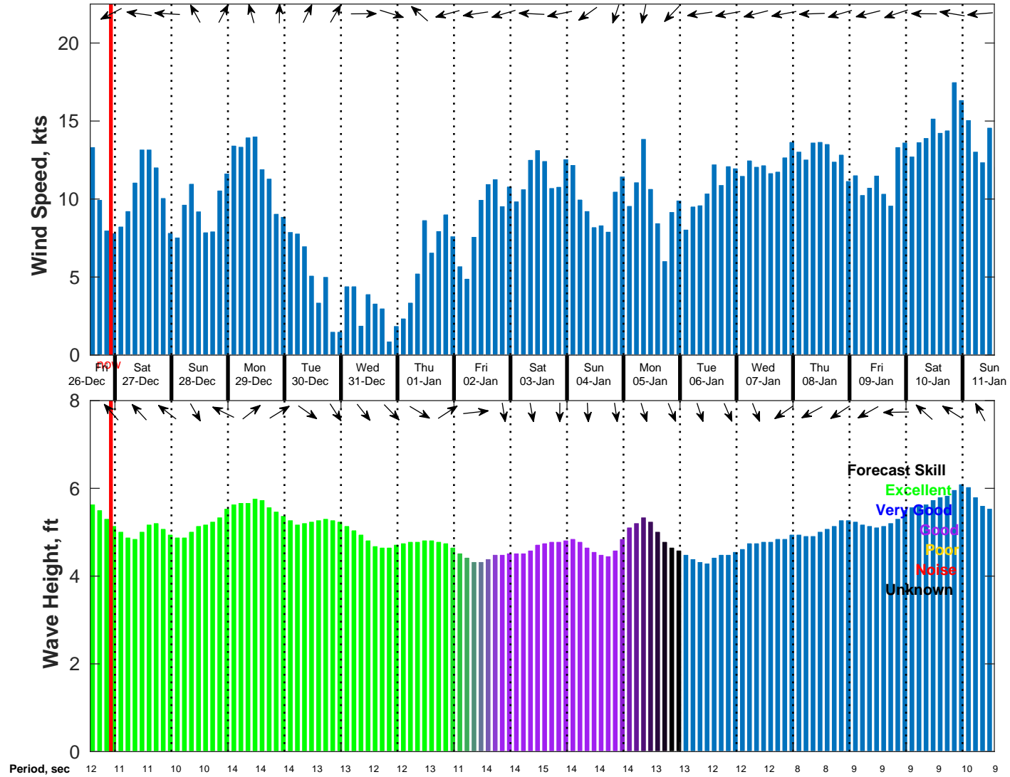
Wind & Wave Forecast for NDBC 51209 from 26-Dec-2025 13:00:00 to 11-Jan-2026 13:00:00
