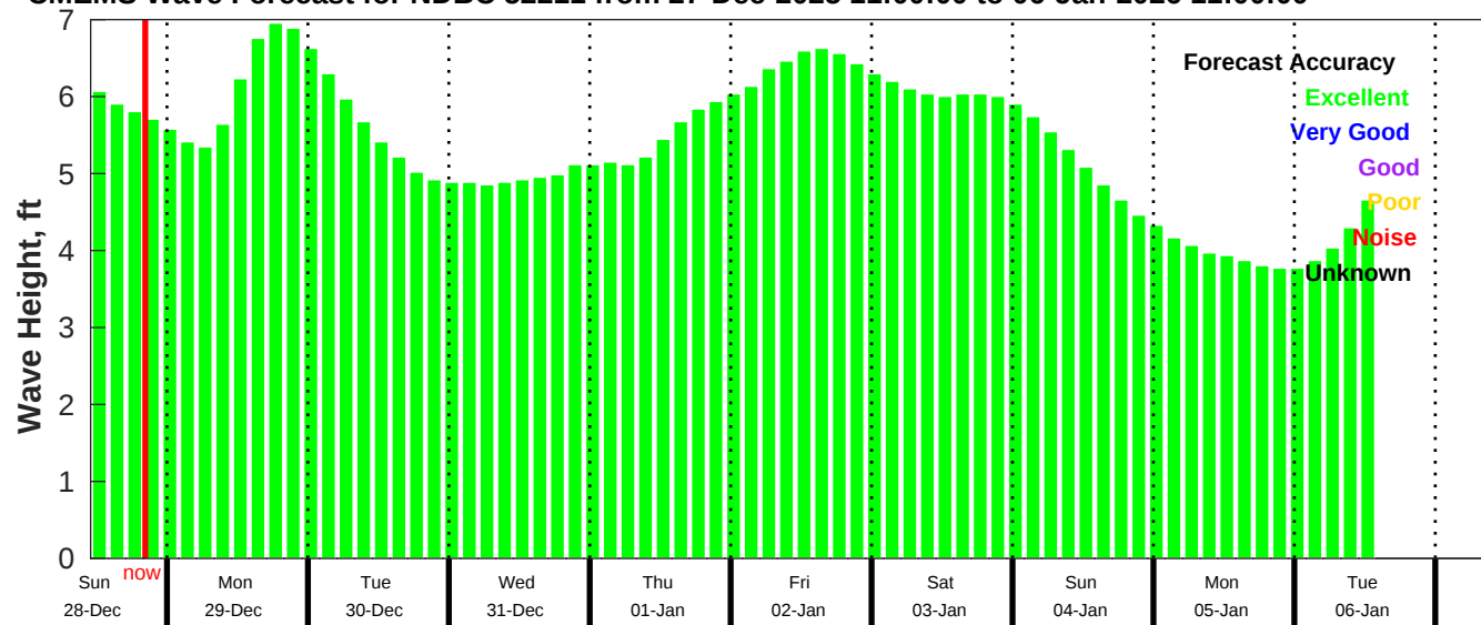
CMEMS Wave Forecast for NDBC 52211 from 27-Dec-2025 11:00:00 to 06-Jan-2026 11:00:00
