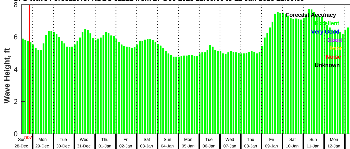
GFS Wave Forecast for NDBC 52211 from 27-Dec-2025 11:00:00 to 12-Jan-2026 11:00:00
