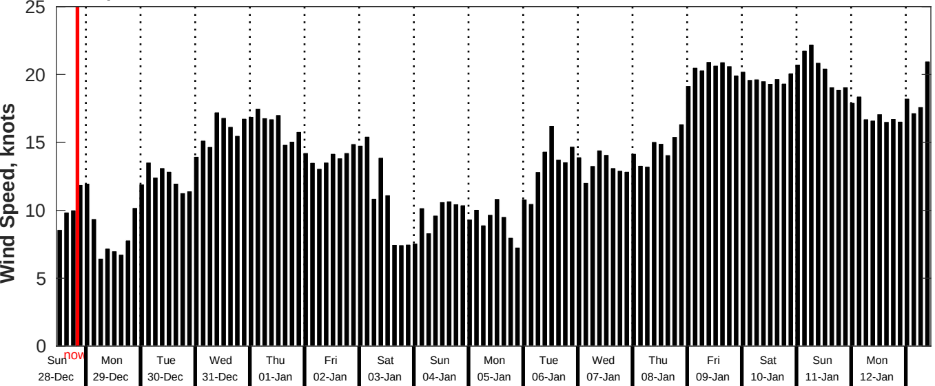
GFS Wind Speed Forecast for NDBC 52211 from 27-Dec-2025 11:00:00 to 12-Jan-2026 11:00:00
