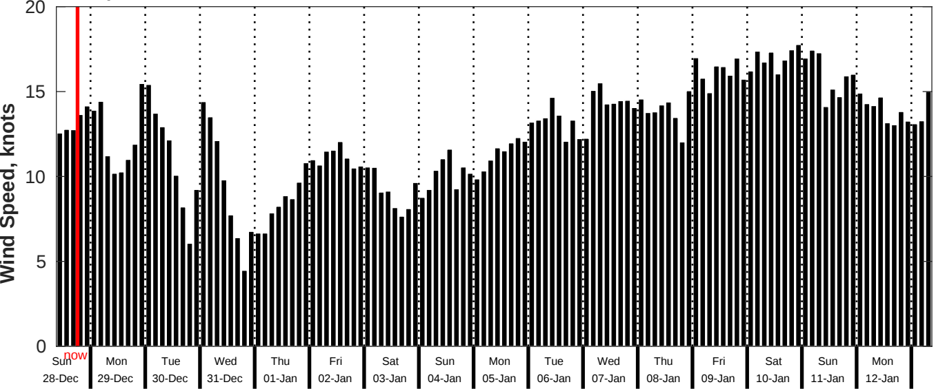
GFS Wind Speed Forecast for NDBC 52212 from 27-Dec-2025 09:00:00 to 12-Jan-2026 09:00:00
