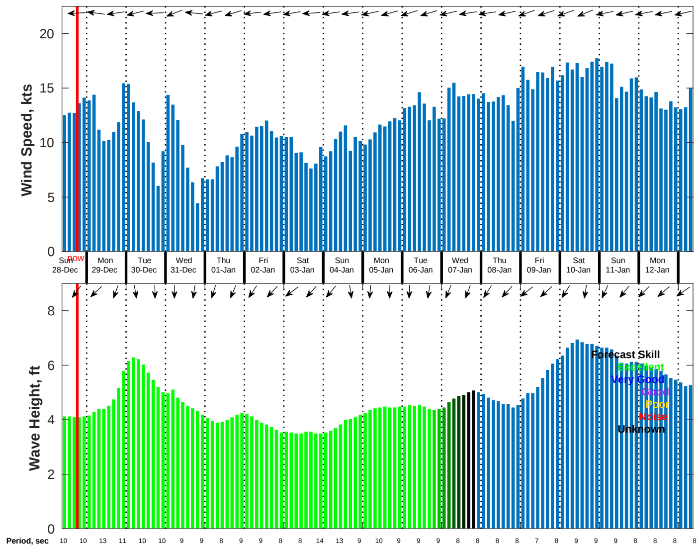
Wind & Wave Forecast for NDBC 52212 from 27-Dec-2025 09:00:00 to 12-Jan-2026 09:00:00
