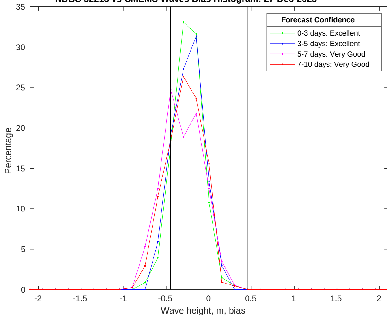
NDBC 52213 vs CMEMS Waves Bias Histogram: 27-Dec-2025
