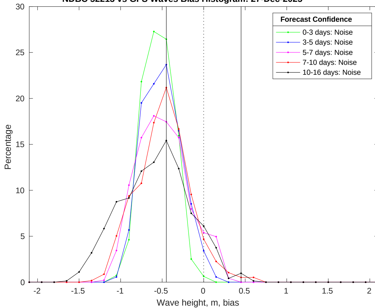
NDBC 52213 vs GFS Waves Bias Histogram: 27-Dec-2025
