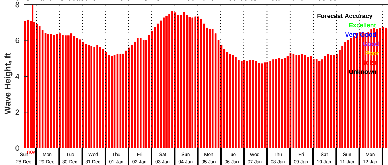
GFS Wave Forecast for NDBC 52213 from 27-Dec-2025 11:00:00 to 12-Jan-2026 11:00:00
