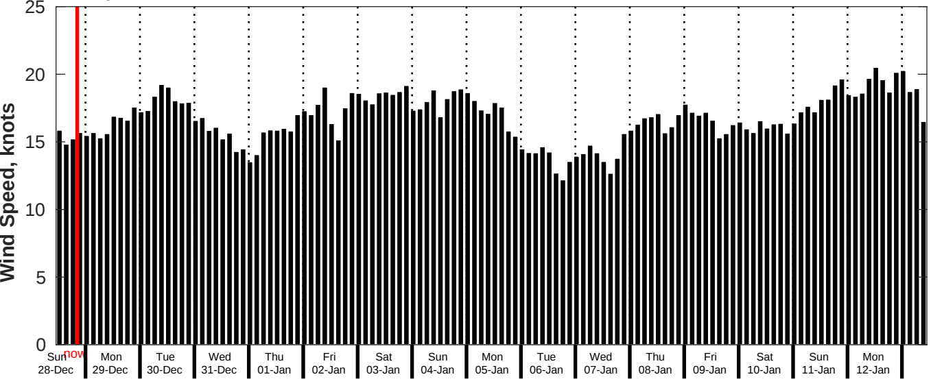
GFS Wind Speed Forecast for NDBC 52213 from 27-Dec-2025 11:00:00 to 12-Jan-2026 11:00:00
