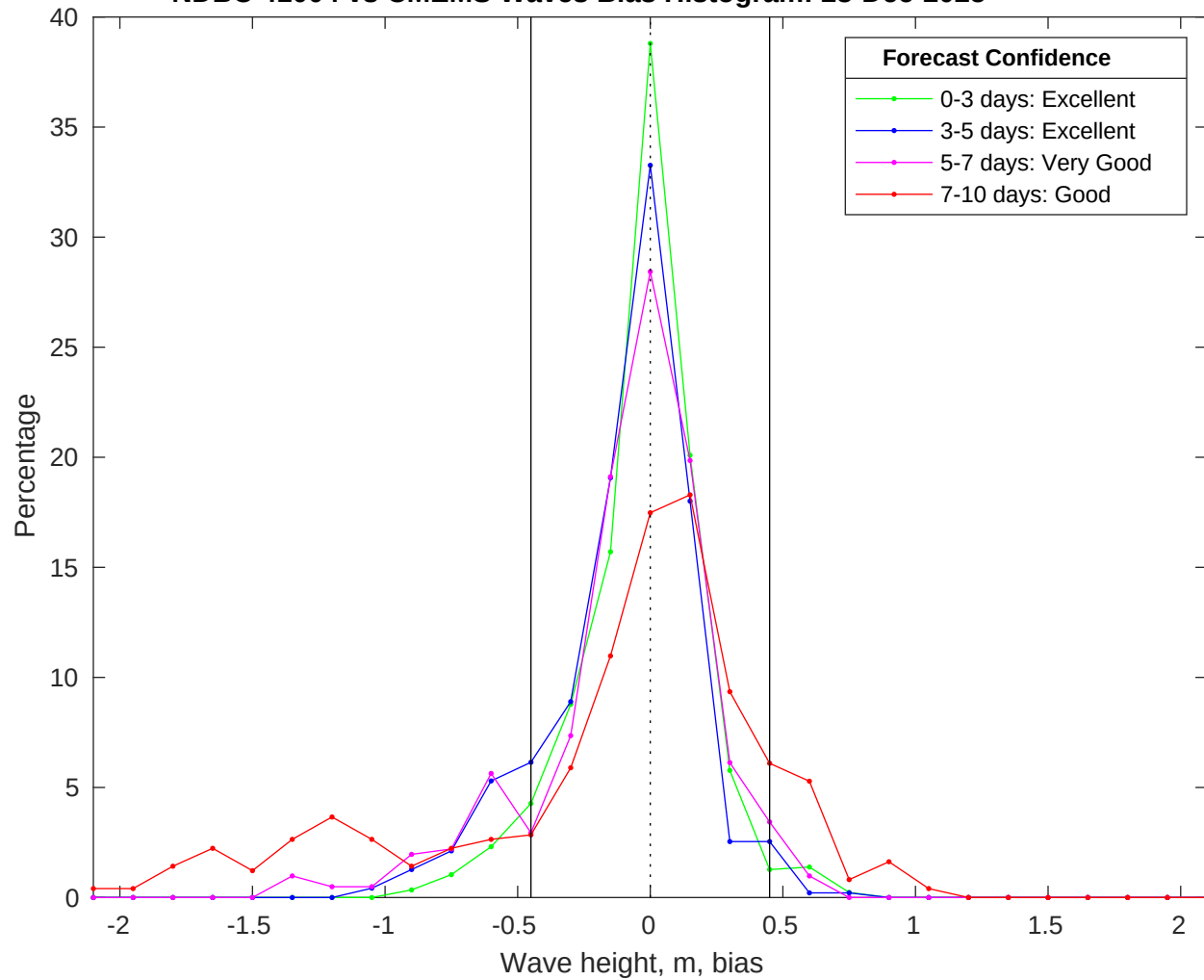
NDBC 41004 vs CMEMS Waves Bias Histogram: 28-Dec-2025
