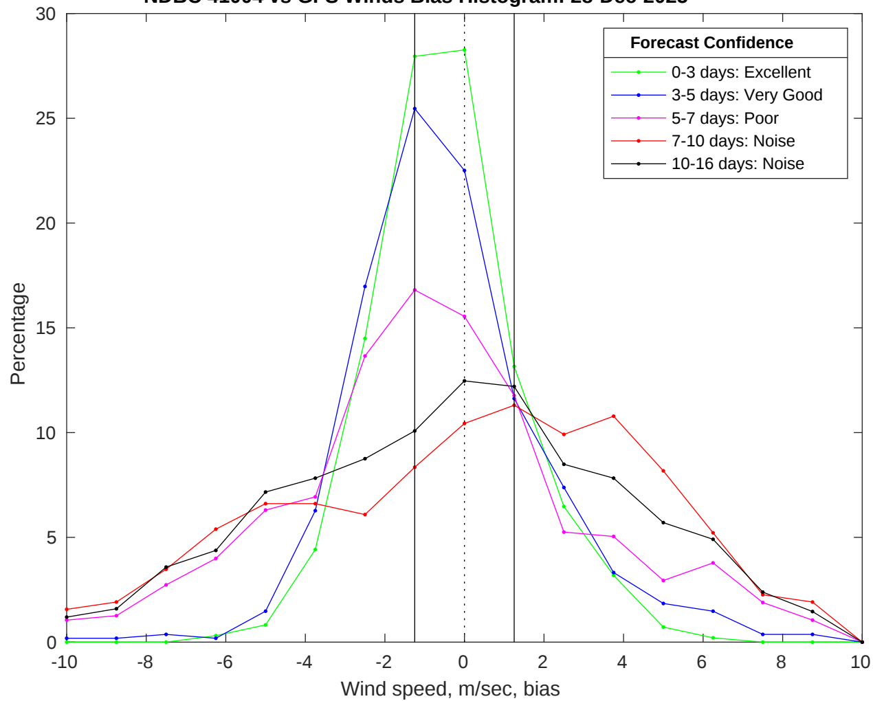
NDBC 41004 vs GFS Winds Bias Histogram: 28-Dec-2025
