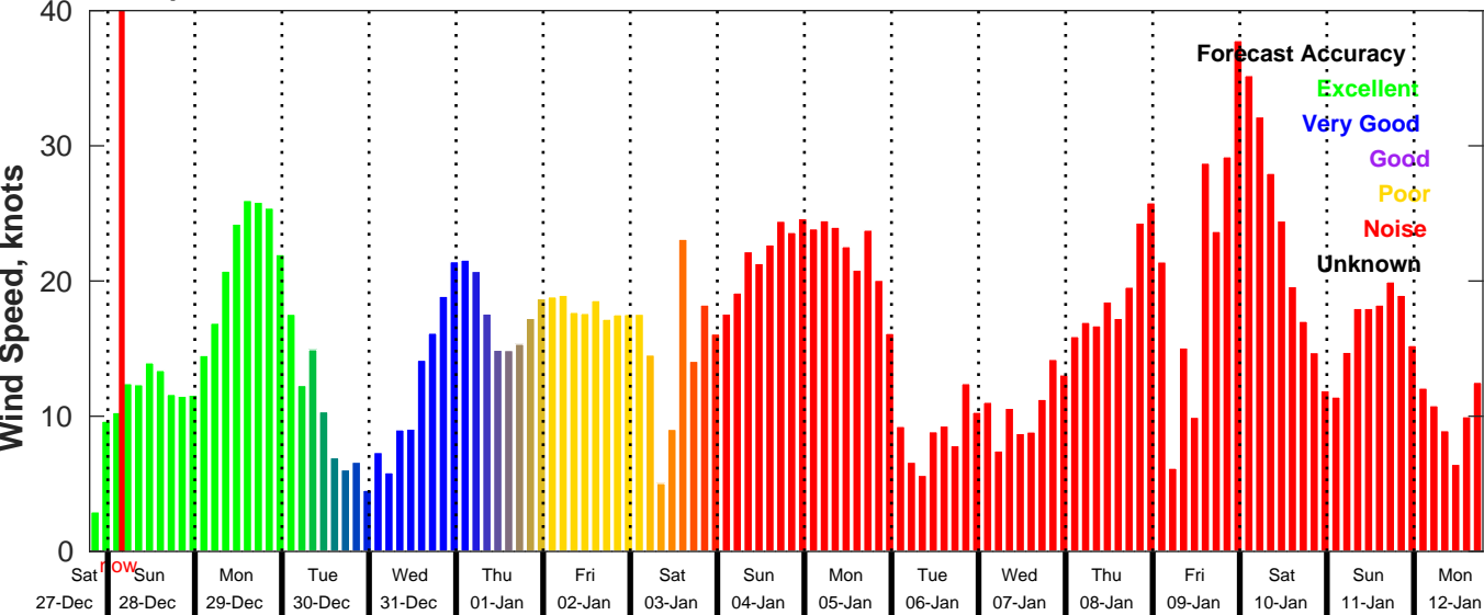
GFS Wind Speed Forecast for NDBC 41004 from 27-Dec-2025 19:00:00 to 12-Jan-2026 19:00:00
