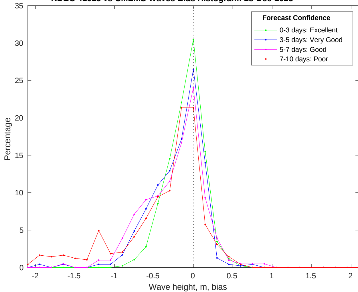
NDBC 41013 vs CMEMS Waves Bias Histogram: 28-Dec-2025
