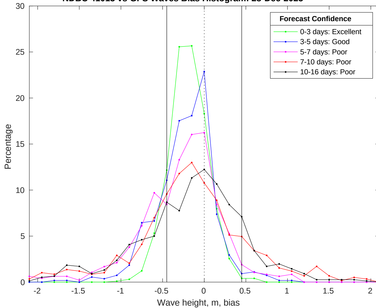
NDBC 41013 vs GFS Waves Bias Histogram: 28-Dec-2025
