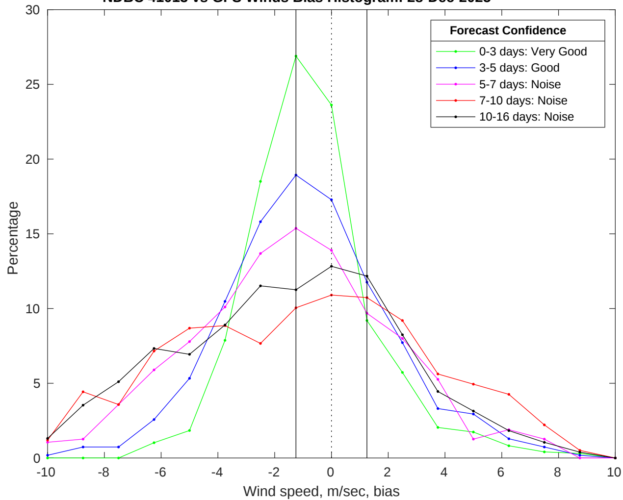
NDBC 41013 vs GFS Winds Bias Histogram: 28-Dec-2025
