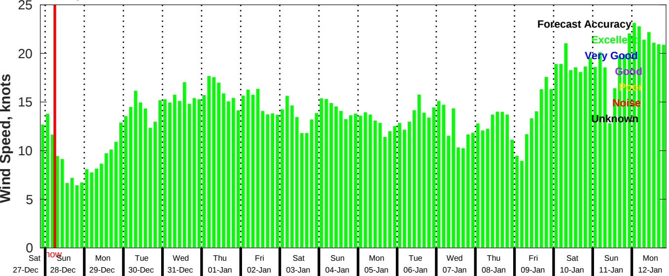
GFS Wind Speed Forecast for NDBC 41040 from 27-Dec-2025 21:00:00 to 12-Jan-2026 21:00:00
