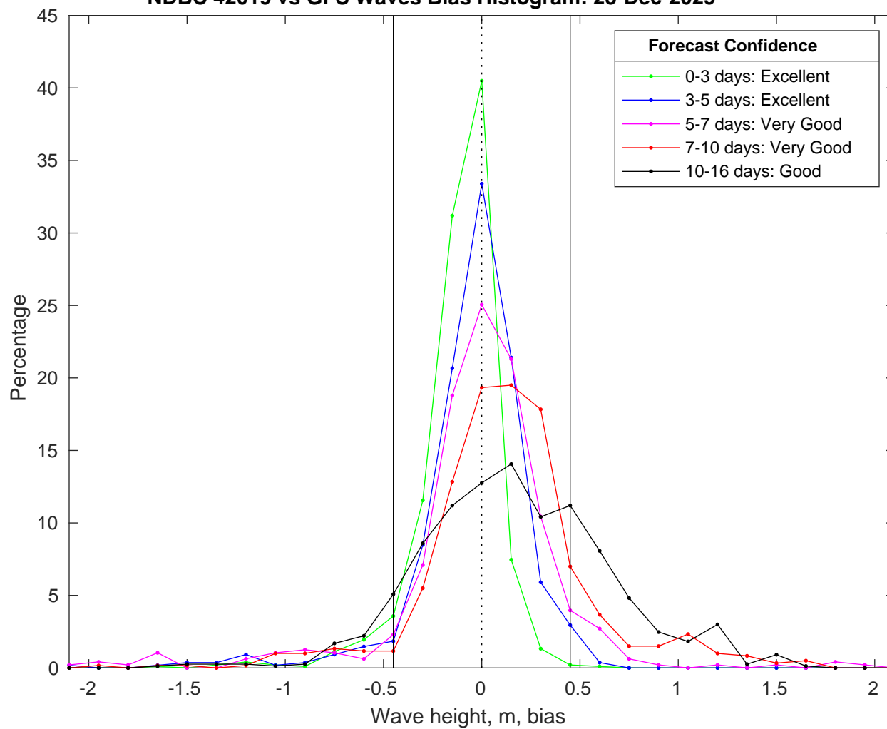
NDBC 42019 vs GFS Waves Bias Histogram: 28-Dec-2025
